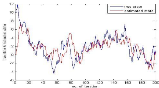
FIGURE 4.3: Number of iteration and true state & estimated state
